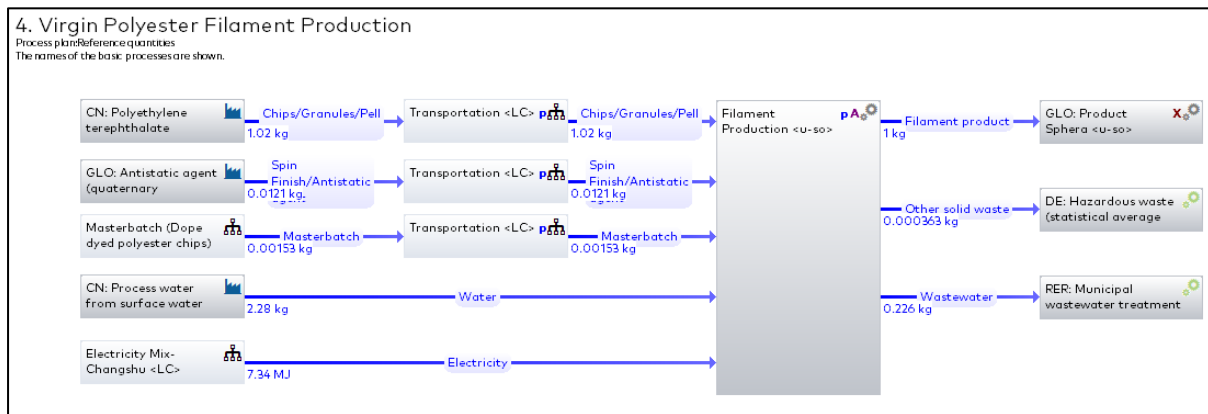
Figure 3-2 LCA FE model snapshot of Virgin Polyester Filament Production from Filament manufacturing
