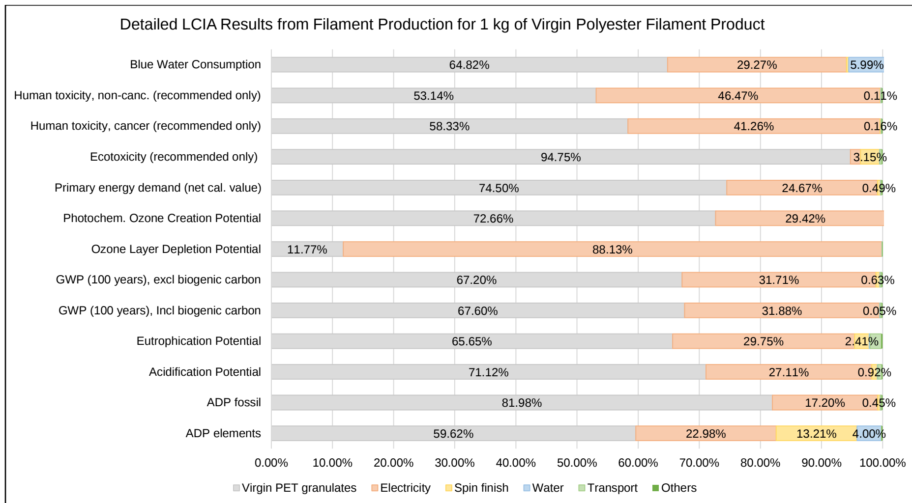
Figure 4-1 Detailed LCIA Results from Filament Production Process for Virgin Polyester Filament Product.
